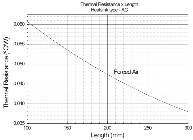
Fig.1 -Thermal resistance
