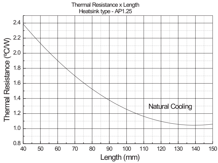
Fig.1 -Thermal resistance
