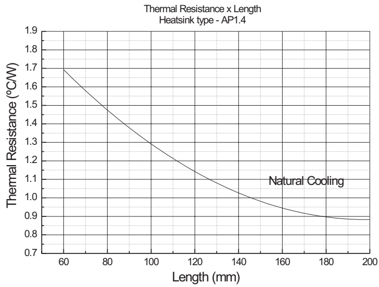
Fig.1 -Thermal resistance
